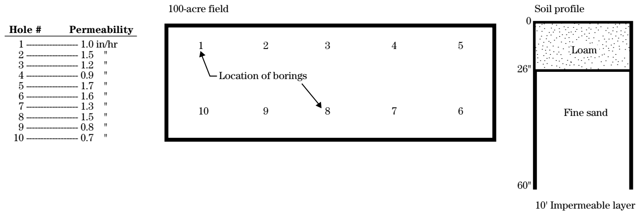
Figure 10-12 A field that requires few hydraulic conductivity tests (1 per 10 acres)*
