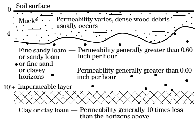
Figure 10-10 Careful consideration for water table control required
