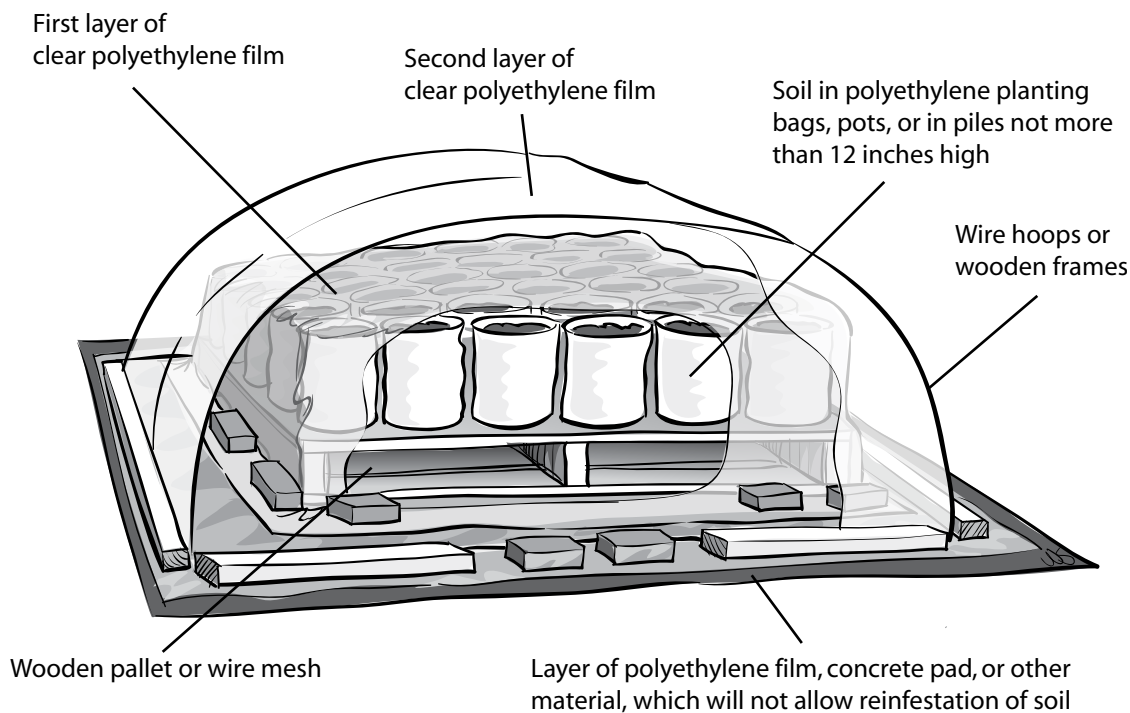
Figure 3. To solarize soil in containers, place soil in buckets or bags on an elevated surface and cover with a double tent of two layers of clear polyethylene film.
